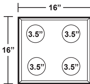
Style PST-3-4
